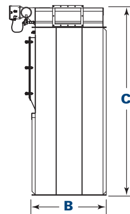
Side View 25FS8 Bin Vent
