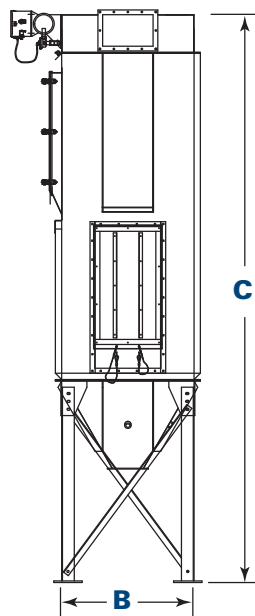
Side View 25FS8
