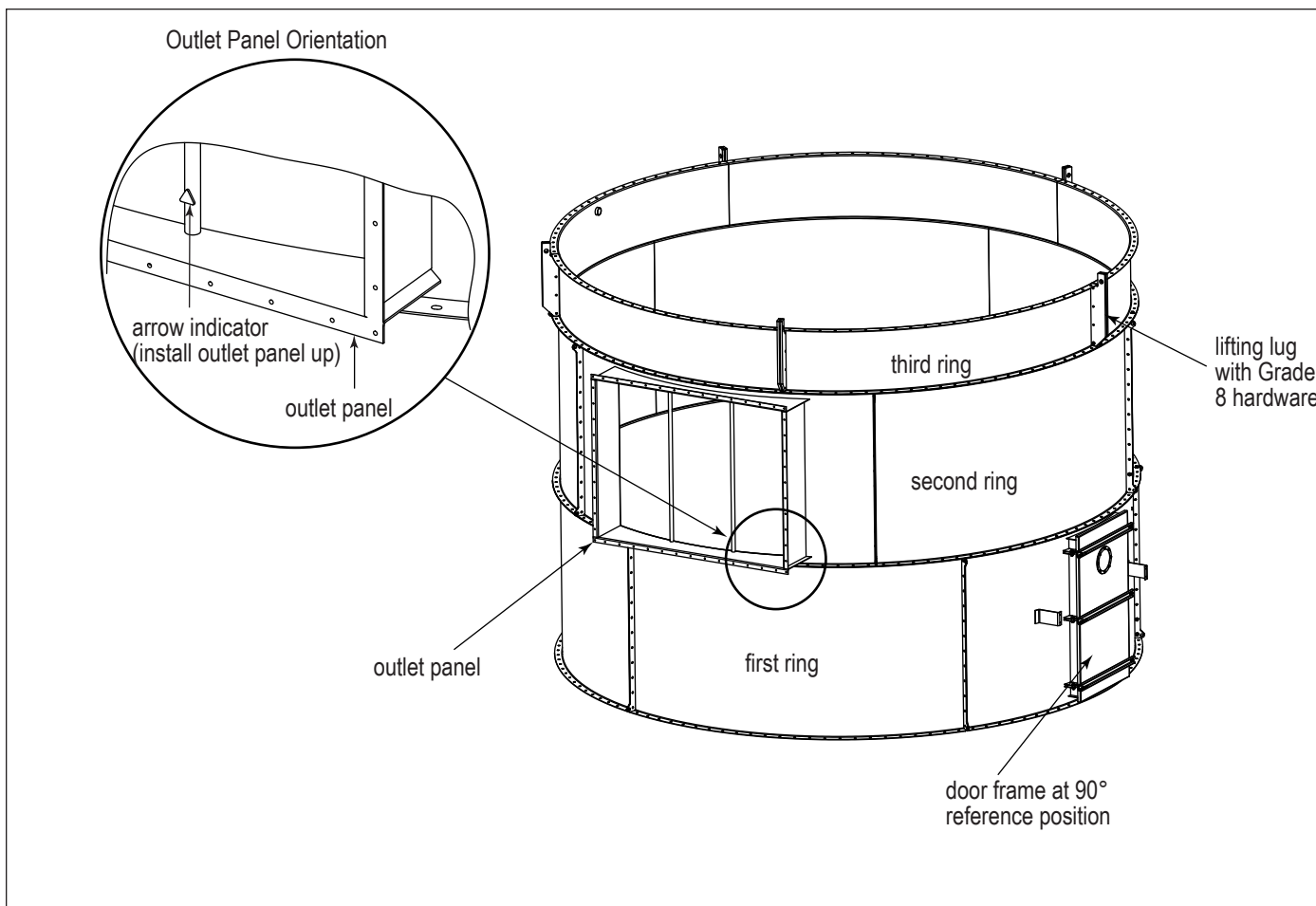
Clean Air Plenum (12-ft Bag Clean Air Plenum Shown)
