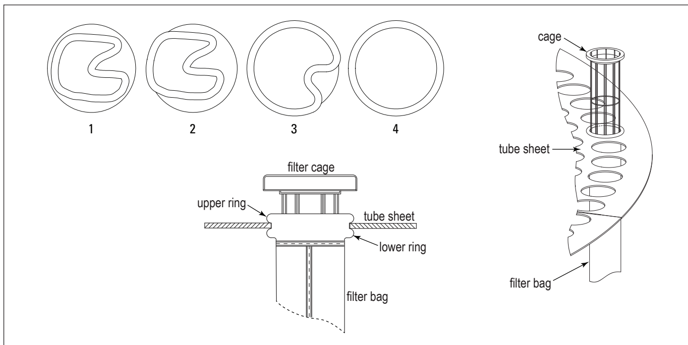
Filter Bag Installation
