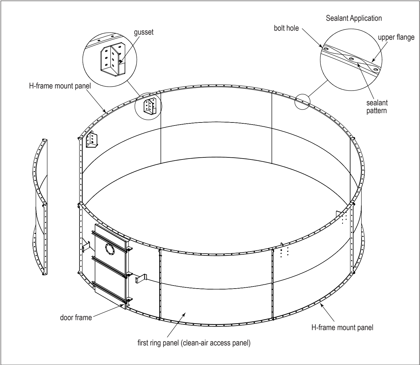
Clean-Air Access Plenum Assembly
