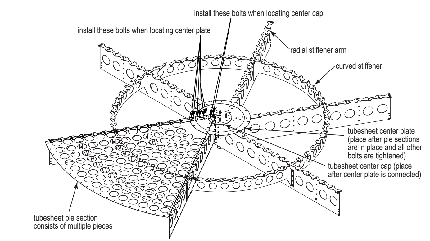
Tubesheet Connection Layout
