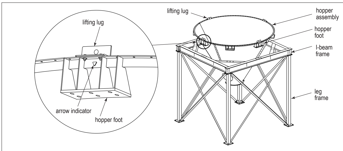
Hopper to Leg Frame Installation
