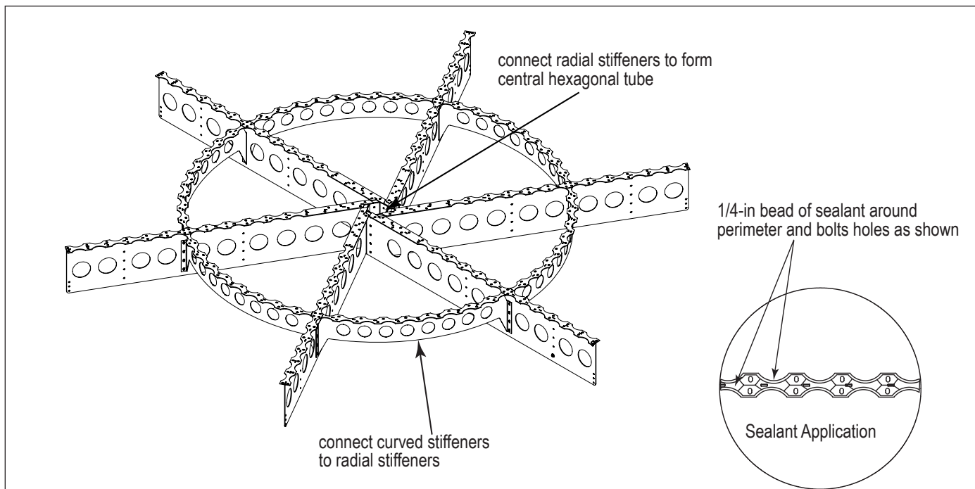
Tubesheet Stiffener Connection and Sealant
