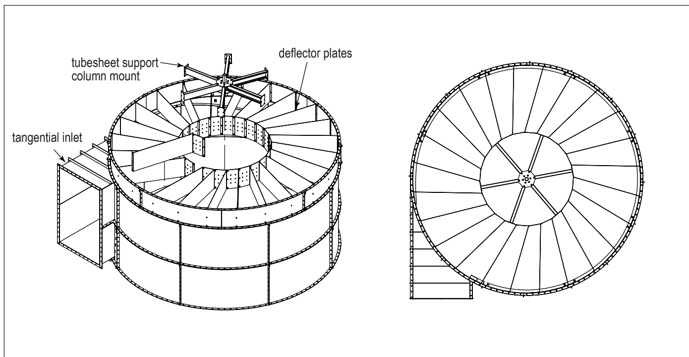
Tangential Inlet
