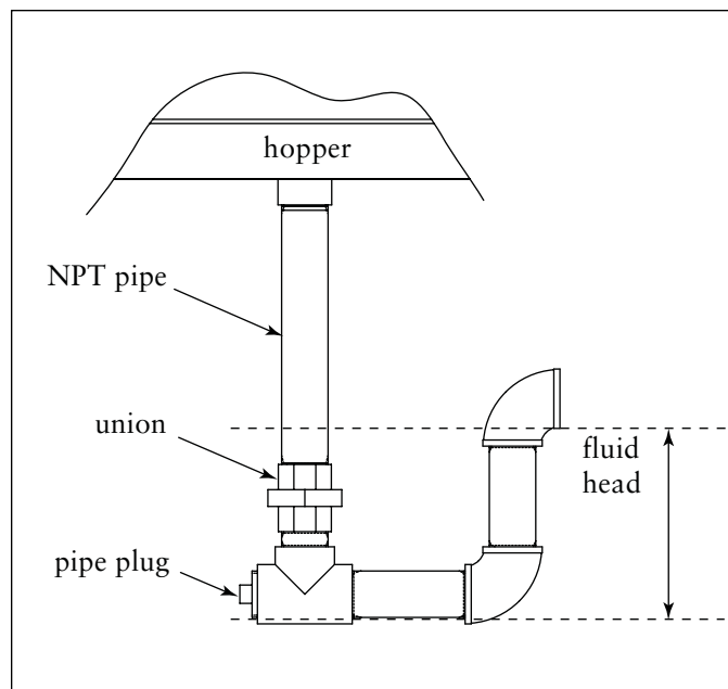
P-Trap Installation
