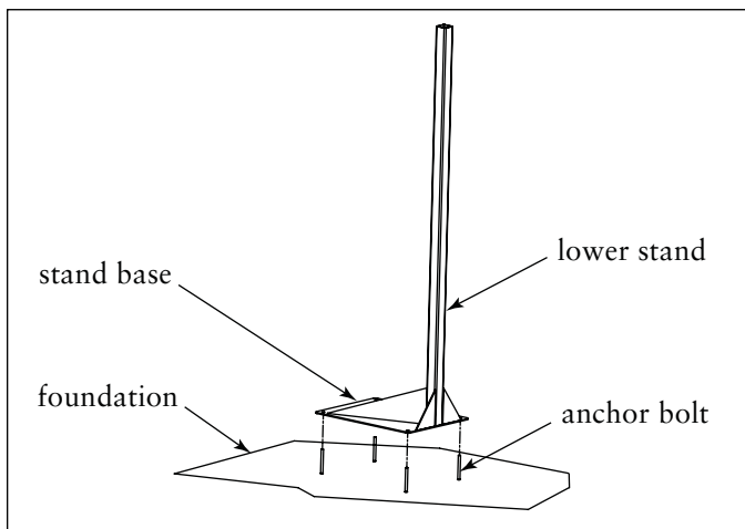
Stand Base Installation, WSO 15 shown
