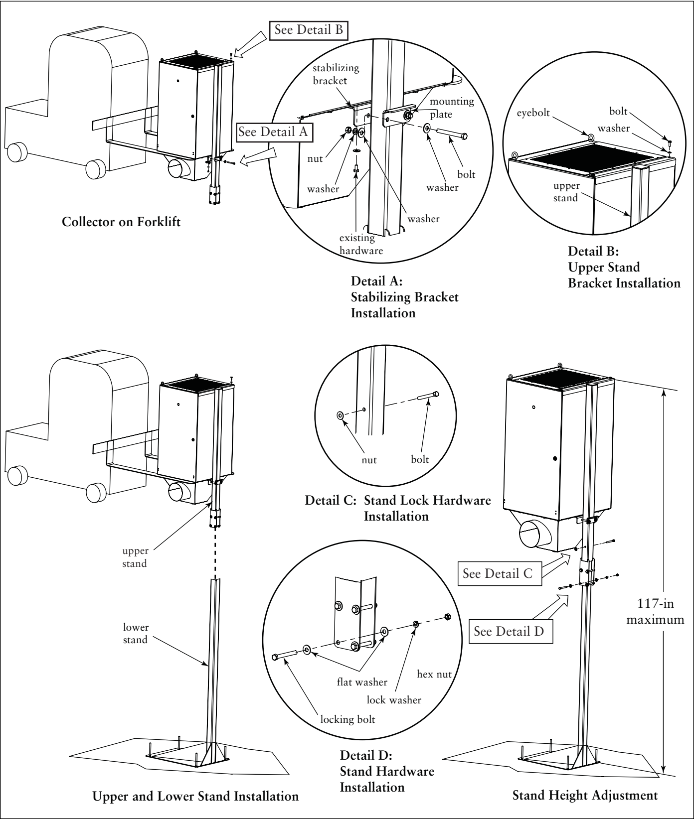
Collector Stand Installation, WSO 15 shown
