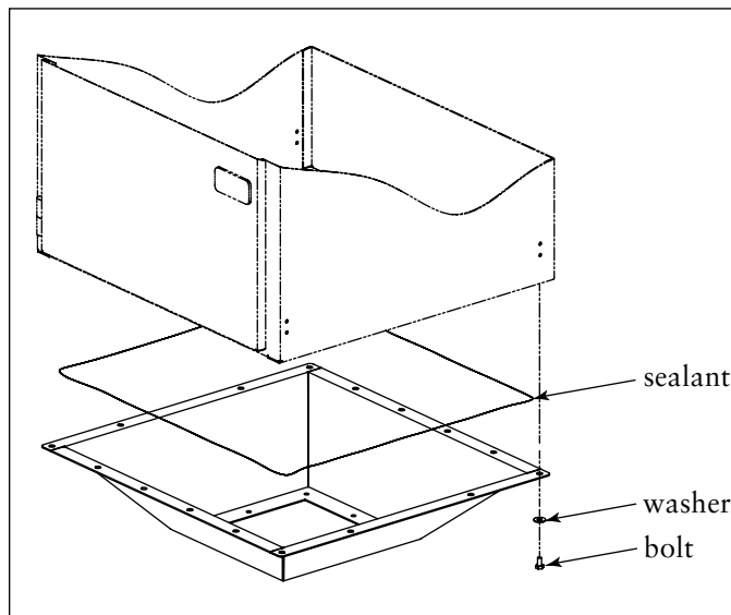
Flanged Inlet Hopper Installation, WSO 15 shown
