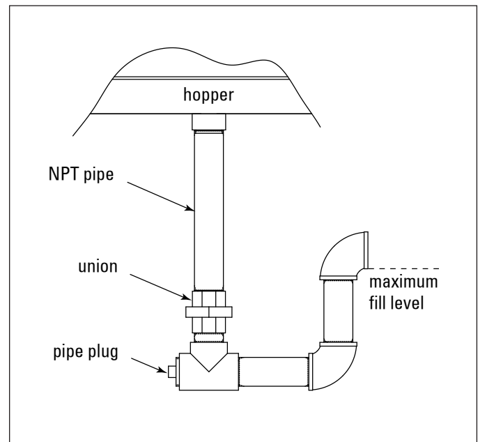
P-Trap Installation
