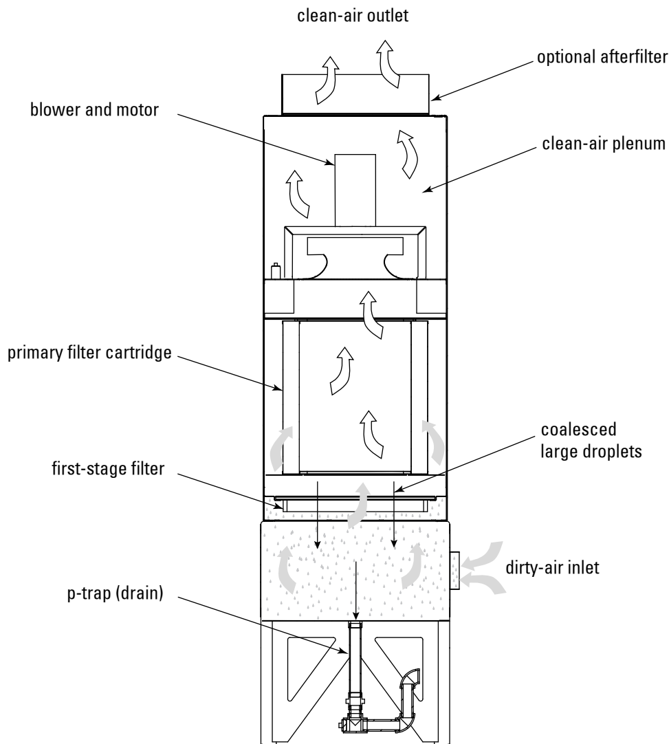
Collector Operation, WSO 25-1 shown
