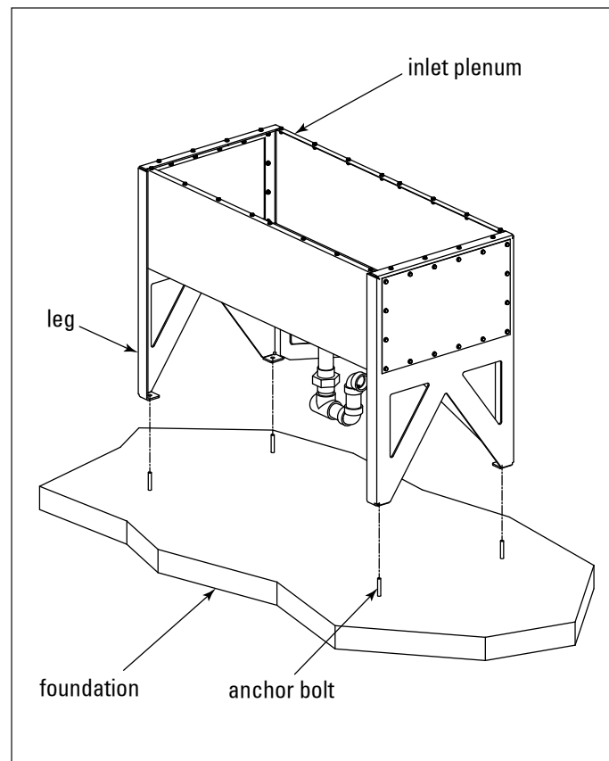
Inlet Plenum Installation, WSO 25-2 shown
