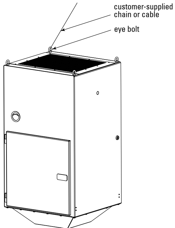
Isometric View
