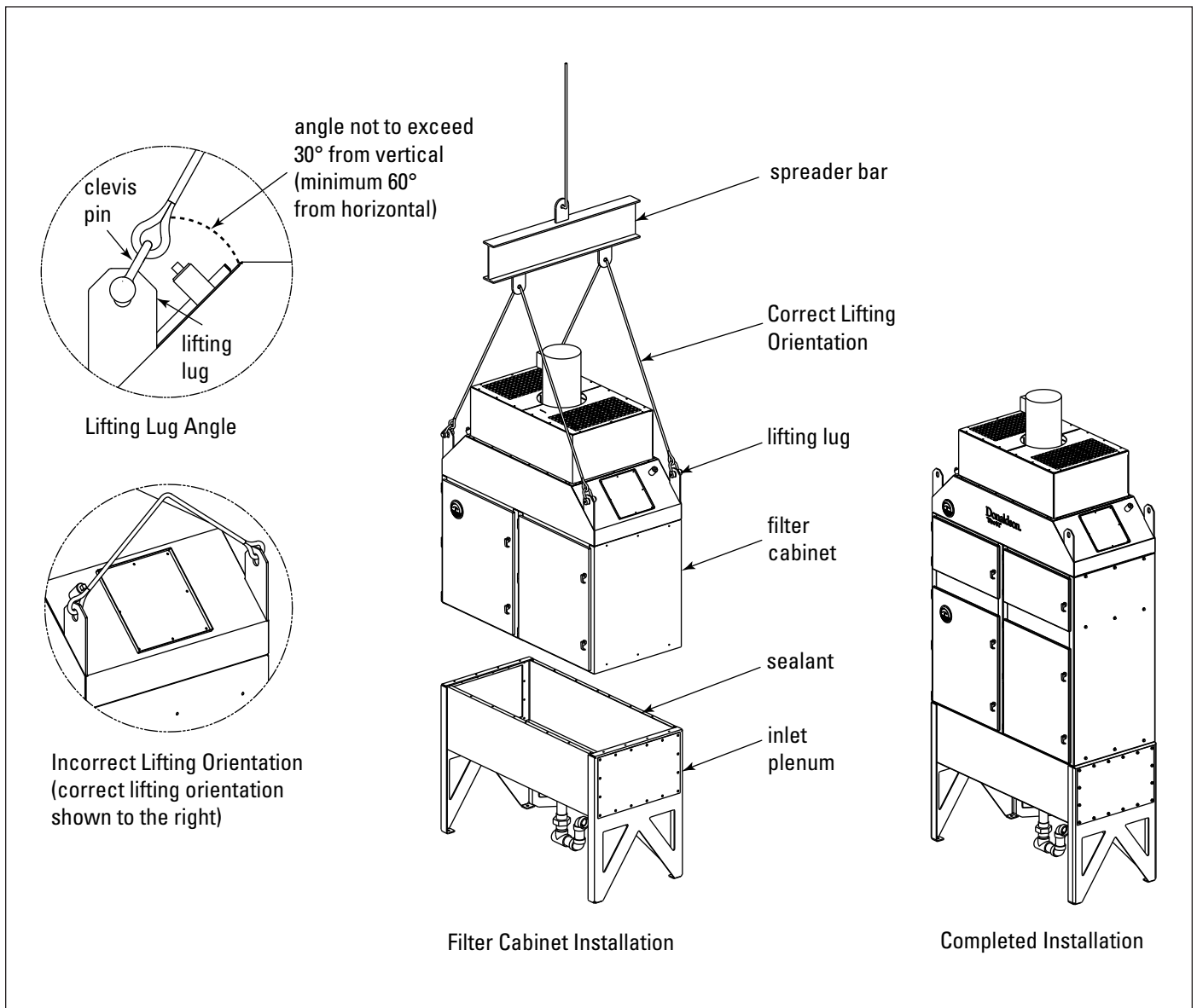
Completed Installation, Powered WSO 25-2 shown
